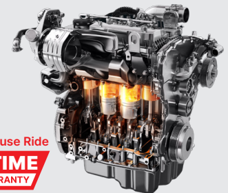
2.3L Puma Diesel Engine with 177 Ps and 450 N-m (A/T)
